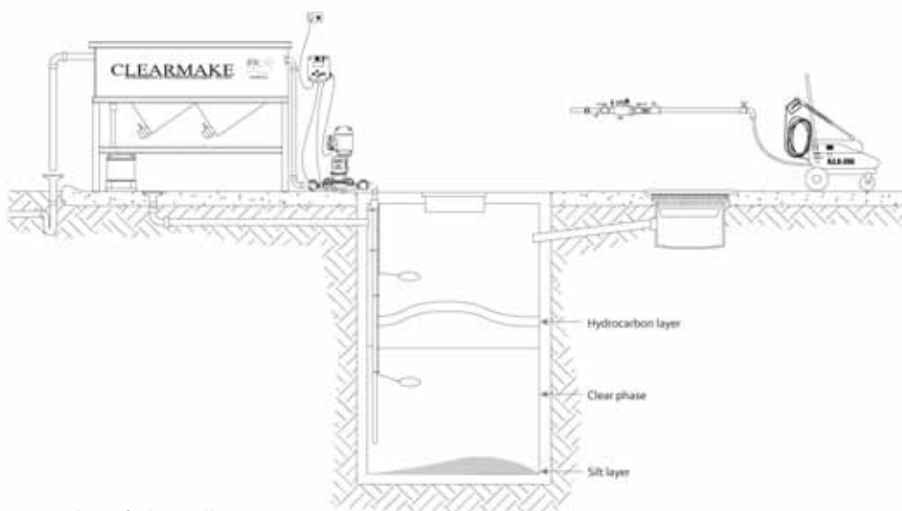
Typical Roofed Installation
